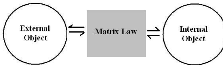
Figure 2.3 Self-interaction between external and internal objects of a quantum entity in a dual universe comprised of an external spacetime and an internal energy-momentum space, vice versa .
