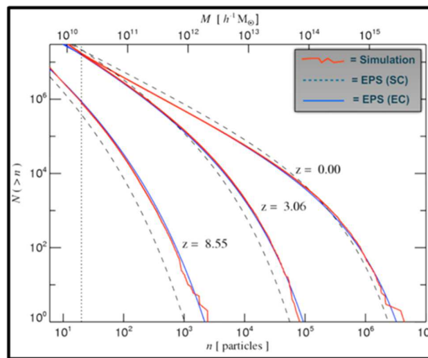
Fig. 1. Scaling behavior of the Press-Schechter theory [10]
