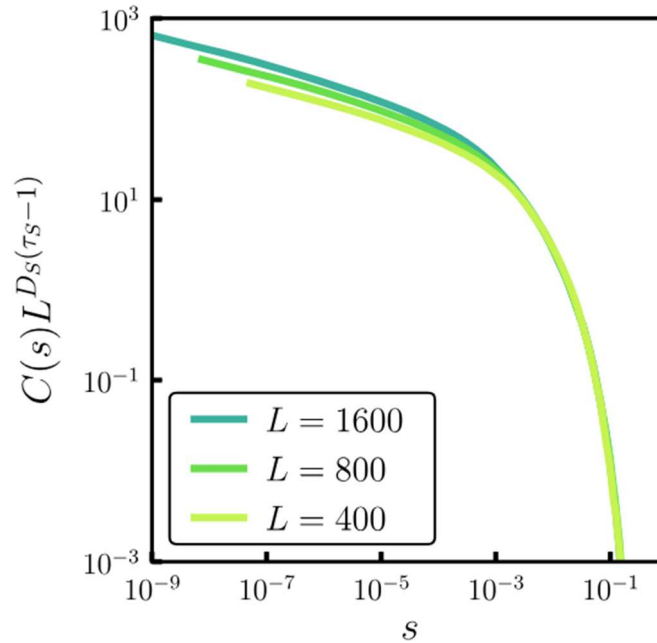
Fig. 2. Scaling behavior of the 2D sandpile model [11-12]
