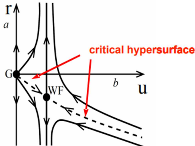
Fig.1: The Gaussian fixed point of scalar field theory
