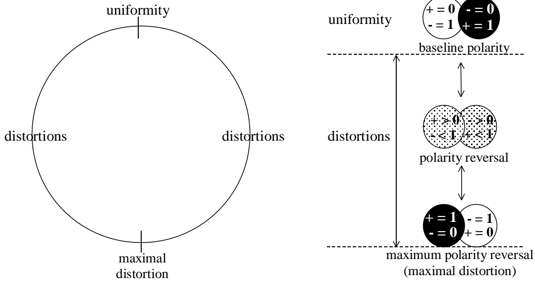
Figure 20 The relationship between the state of uniformity and the degrees of reality-cell distortion with regard to the pattern of content distribution. The maximal reality-cell distortion is the pattern of content distribution that's the exact opposite of the state of uniformity. Between these polar extremes lie an infinite number of intermediate degrees of reality-cell distortion, depicted by shades of gray. Any movement away from the state of uniformity is an increase in reality-cell distortion; any movement away from the maximal distortion is a movement towards the state of uniformity.
