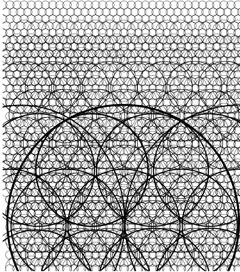
Figure 15 The uniformity and consistency of the structure of the relational matrix occurring both between reality cells at any one relational level of reality, and within reality cells at different relational levels of reality. Depicted here are five relational levels of reality, represented by five different-sized circles representing five different-sized reality cells. At the top, the overlapping levels have been omitted for better visibility of the different relational levels of reality depicted in the diagram.
