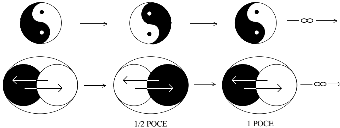
Figure 10 The reality-cell period of content exchange (POCE). Illustrating the cyclic or periodic exchange of spatial content that occurs between the reality cells as they continuously penetrate each other. One full cycle of content exchange is one POCE. The paired arrows represent vectors of reality cell expansion or penetration.
