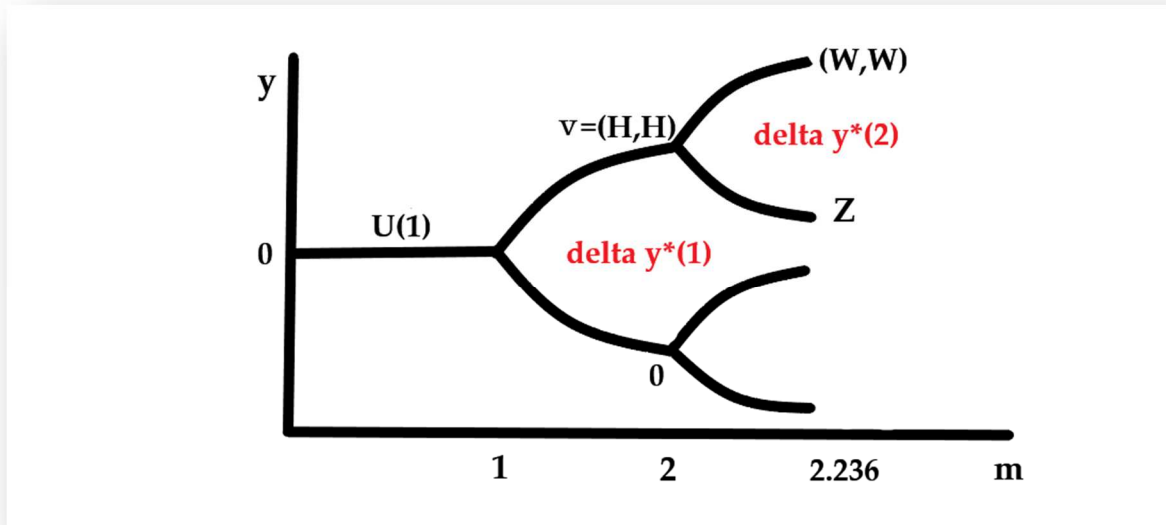
Fig. 1. Bifurcation diagram of the cubic map (16) for \Delta\varphi^*(1) = +v
