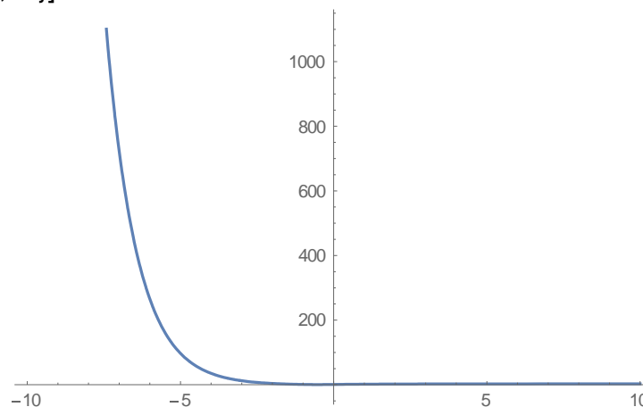
Figure 1. Plot for numerical solution of Ermakov equation
